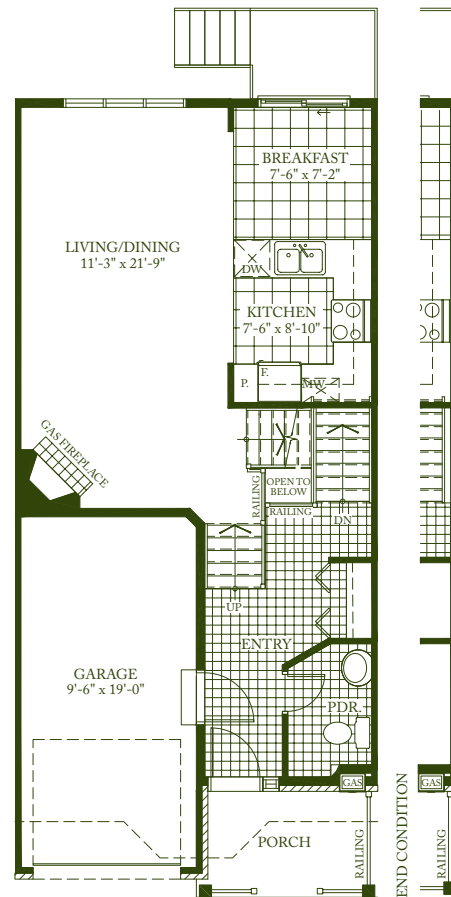
GROUND FLOOR AREA = 585 sq. ft. TOTAL AREA = 1675 sq. ft.
